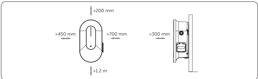
Figure 4-4 Clearance requirement
