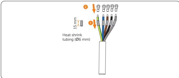
Figure 6-13 Install the tubing and R-type terminal
